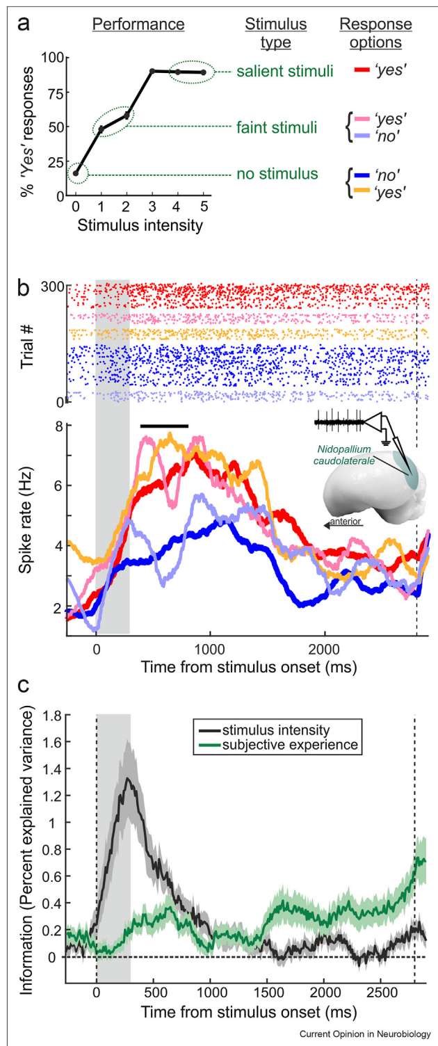
Behavioral performance of a crow and neuronal responses from its NCL related to sensory consciousness. (a) Psychometric functions of a crow performing the rule-based delayed detection task (shown in Fig. 2). Trials were grouped into salient-stimulus, faint-stimulus near-threshold, and no-stimulus trials. The different response options ('yes'/'no') for each trial group are color coded and depicted on the right. Error bars (very small) indicate the standard error of the mean. (b) The activity of an NCL
